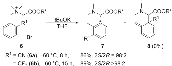
Scheme 2. Asymmetric Sommelet–Hauser rearrangement of ortho -substituted N -benzylic ammonium salt 6 . R^* = (-) -8-phenylmenthyl.
